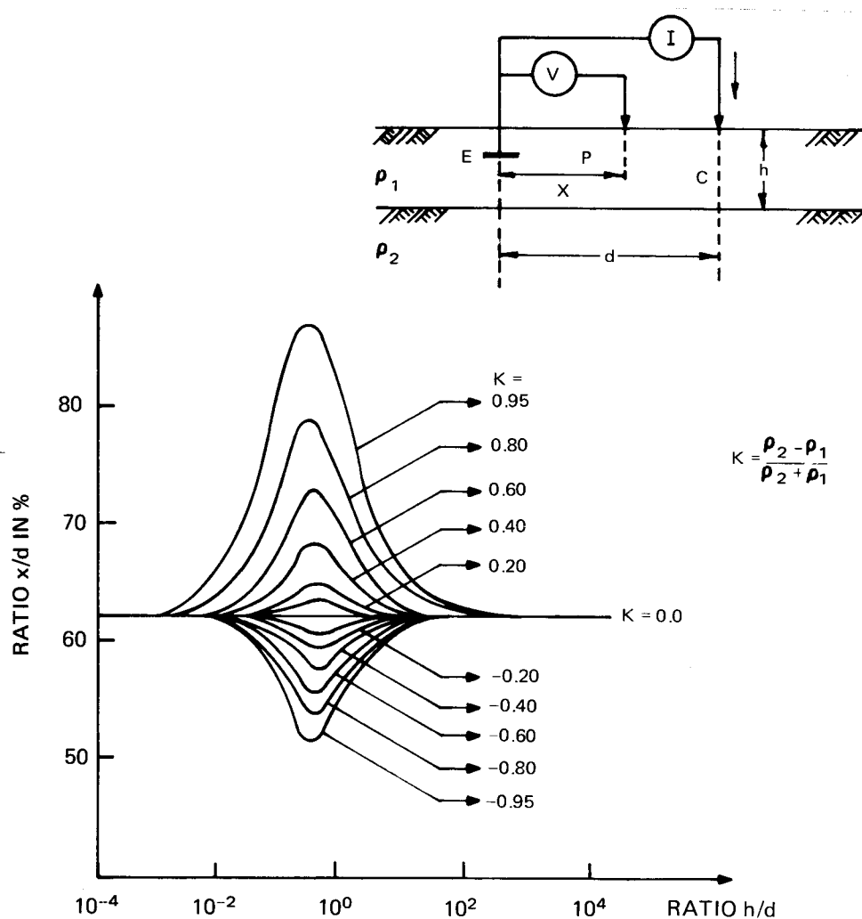
Figure 10—Required Potential Electrode Position in a Two Layer Earth
