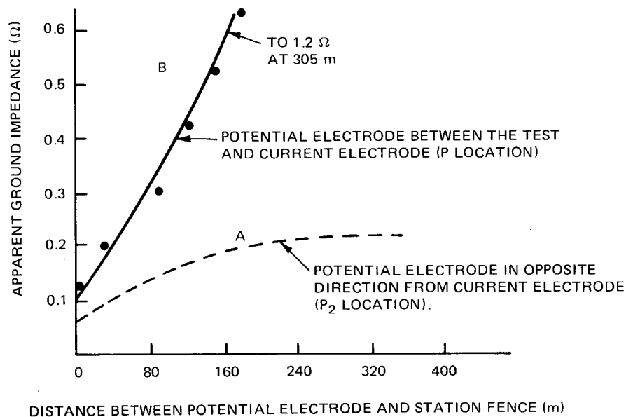
Figure 9—Case of a Low-Impedance Ground System
