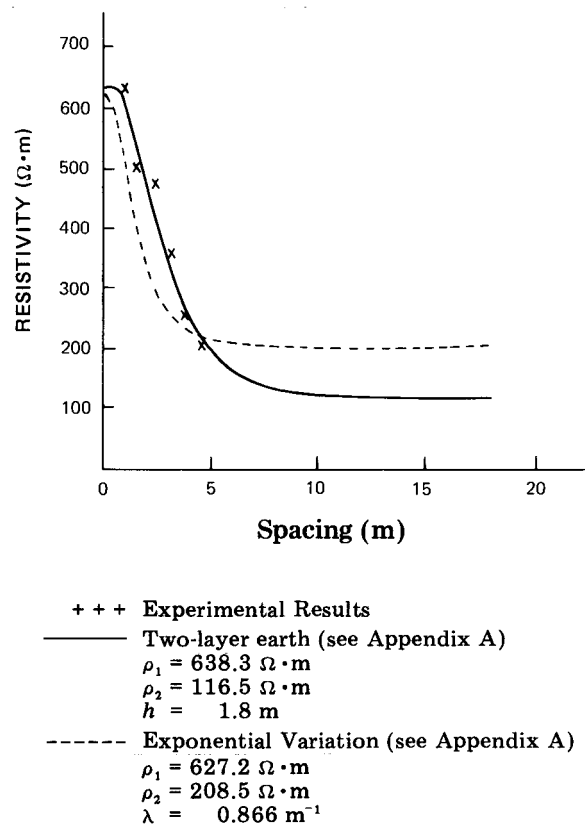
Figure 5—Example of an Earth Resistivity Interpretation
