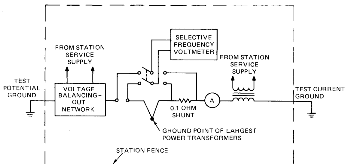
Figure 17—Selective-Frequency Voltmeter-Ammeter Circuit
