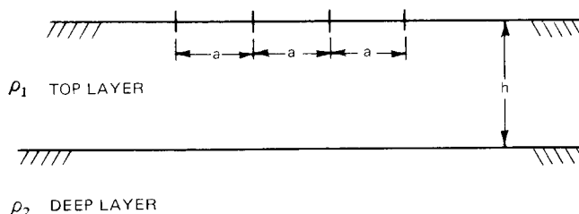
Figure A.1—Two-Layer Earth
