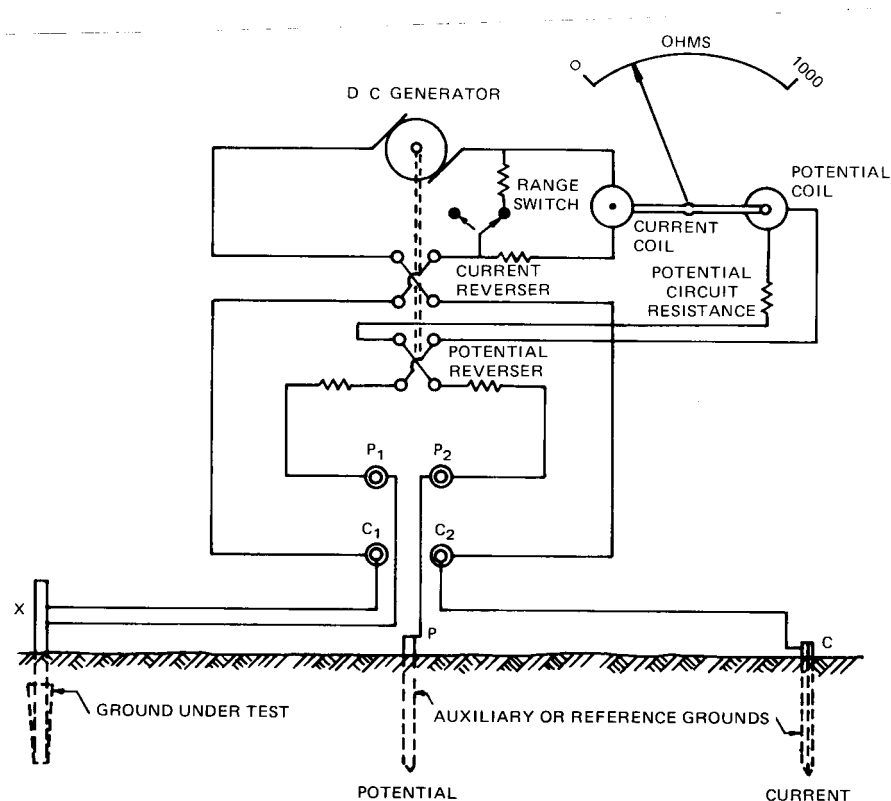
Figure 14—Ratio Ohmmeter
