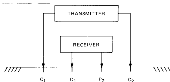
Figure 18—Induced Polarization Units
