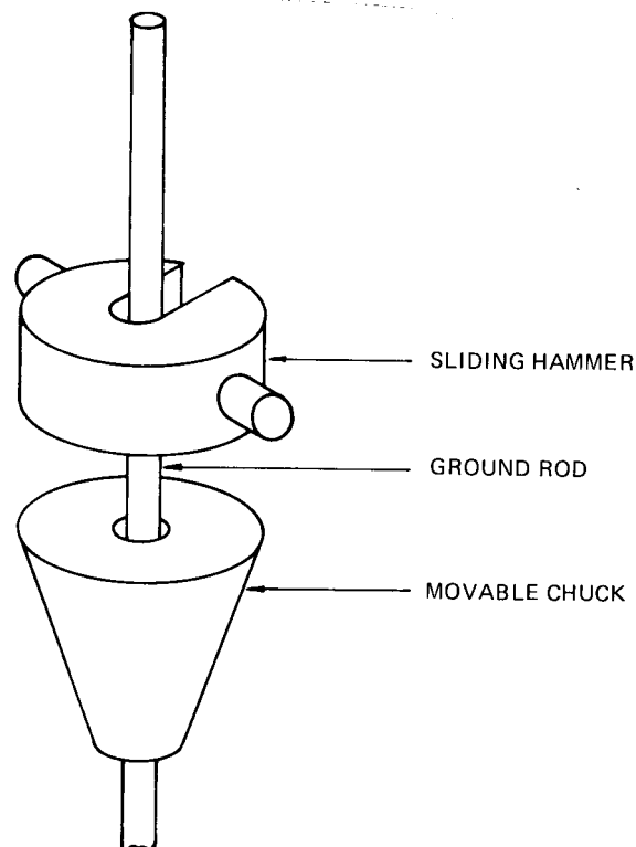
Figure 20—Chuck and sliding Hammer
