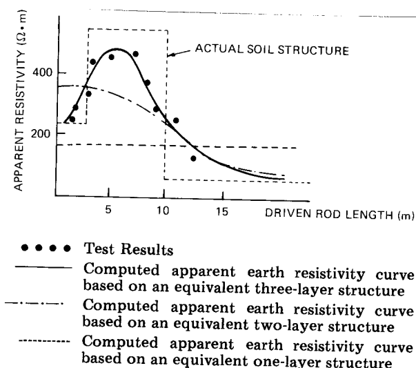
Figure 4—Variation of Depth Results
