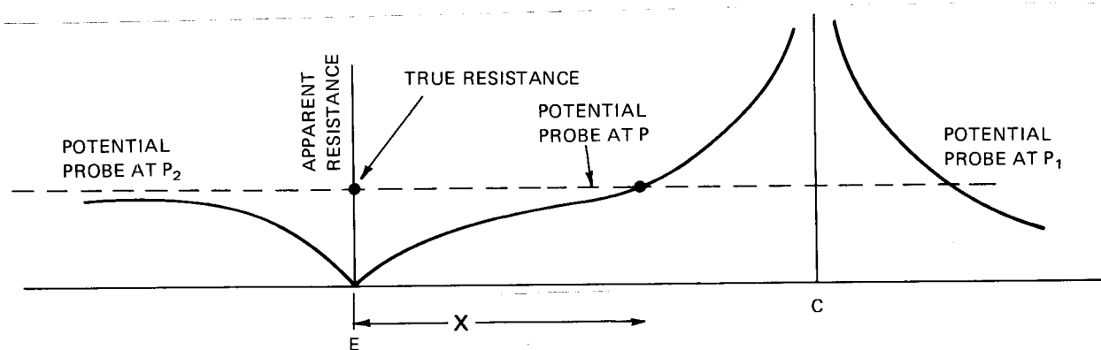
Figure 7—Apparent Resistance for Various Spacings x
