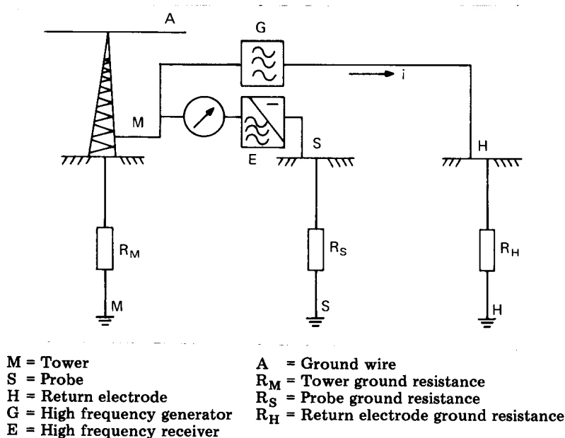
Figure 19—High-Frequency Meter
