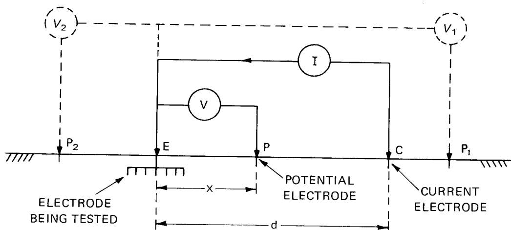
Figure 6—Fall-of-Potential Method
