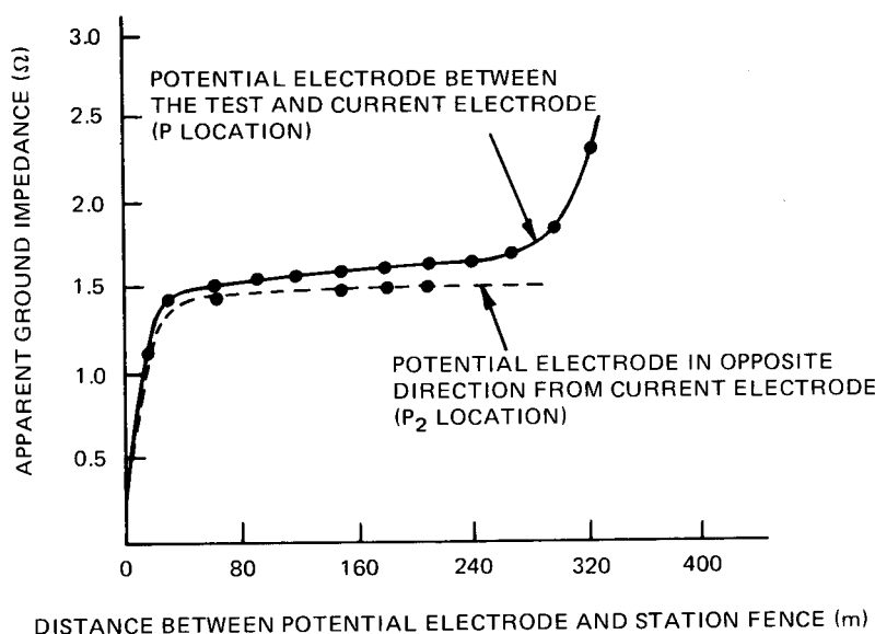
Figure 8—Case of a High-Impedance Ground System
