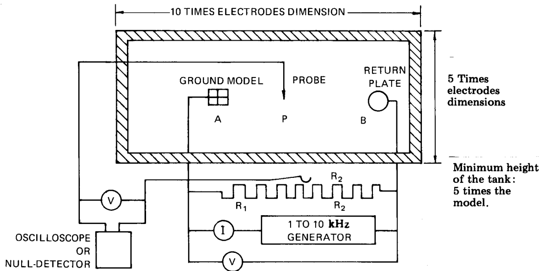
Figure 13—Electrolytic Tank
