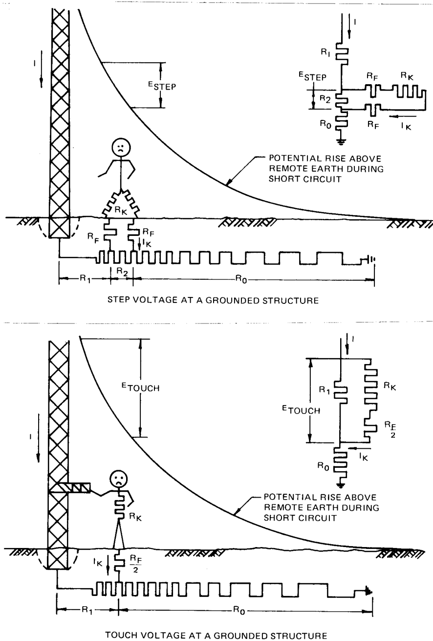
Figure 11—Step and Touch Voltages
