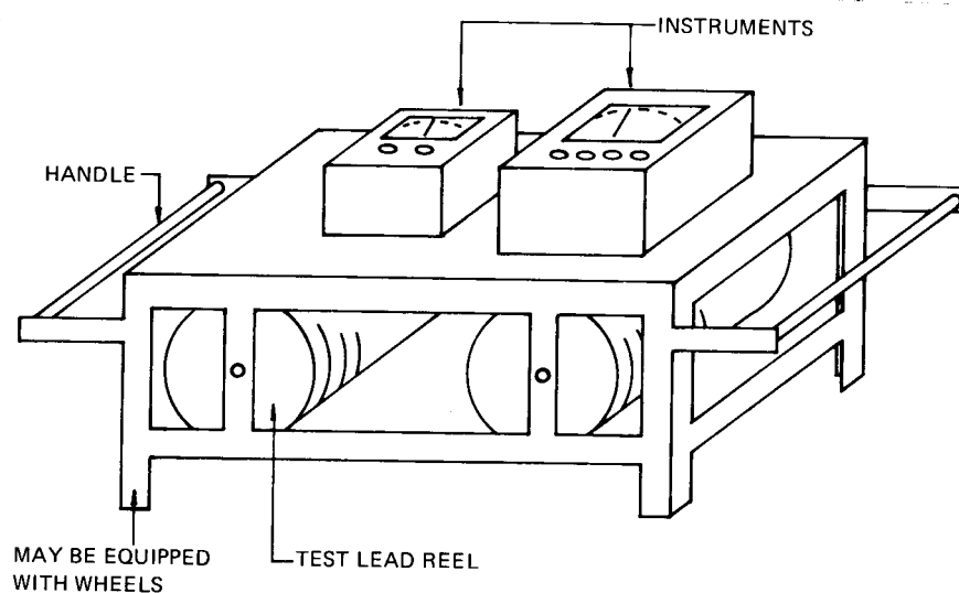
Figure 21—Test Table
