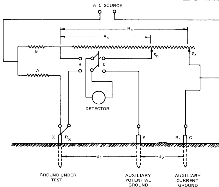
Figure 15—Double-Balance Bridge
