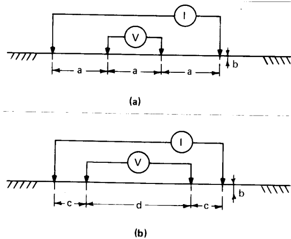
Figure 3—Four-Point Method (a) Equally Spaced (b) Unequally Spaced
