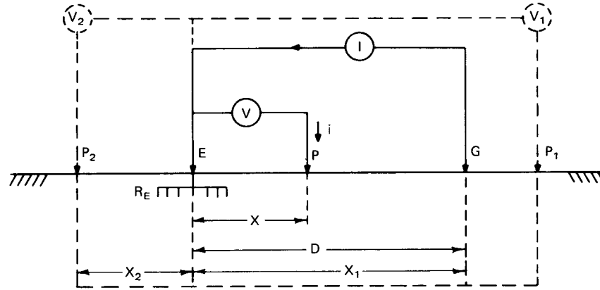
Figure C.1—Fall-of-Potential Method
