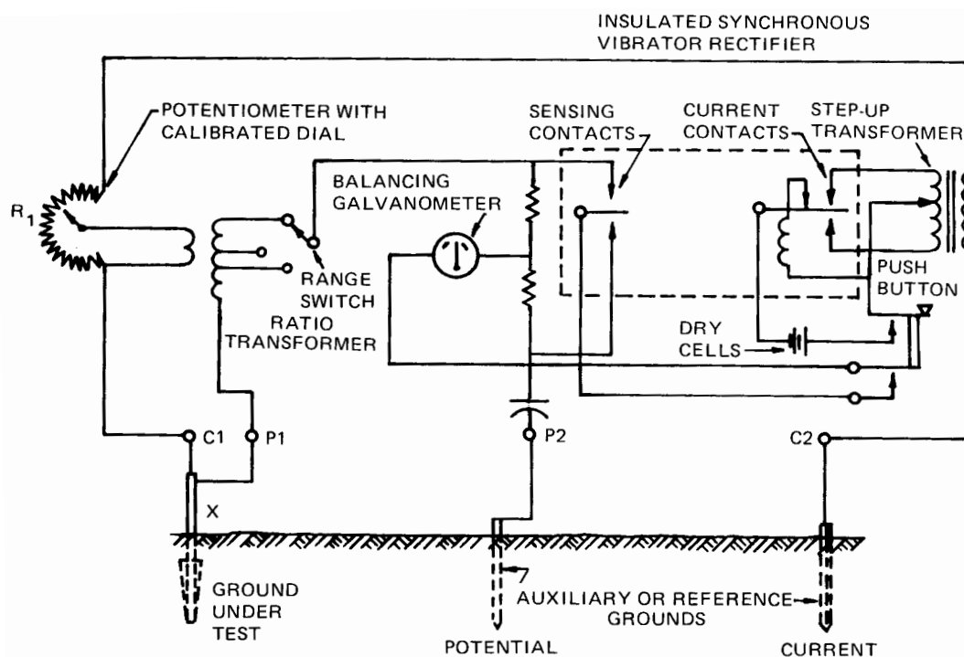
Figure 16—Single-Balance Transformer
